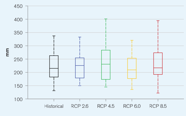
FIGURE 8. The boxplot shows the projected annual average precipitation for Uzbekistan in the period 2080–2099. 22
