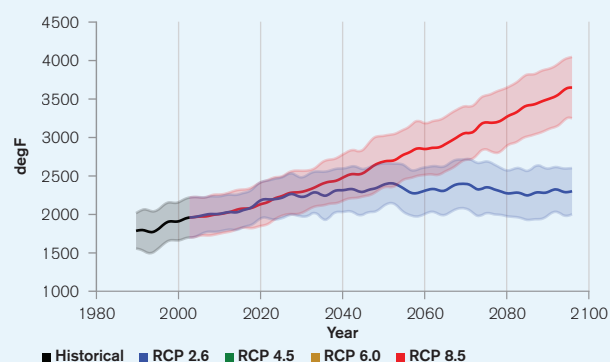
FIGURE 13. Historic and projected annual cooling degree days in Uzbekistan (cumulative degrees above 65°F) under RCP2.6 (blue) and RCP8.5 (red). The values shown represent the median of 30+ GCM model ensemble with the shaded areas showing the 10–90th percentiles. 22
