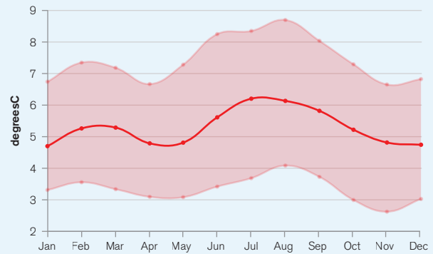
FIGURE 7. Projected change (anomaly) in monthly temperature, shown by month, for Uzbekistan for the period 2080–2099 under RCP8.5. The value shown represents the median of the model ensemble with the shaded areas showing the 10th–90th percentiles. 22
